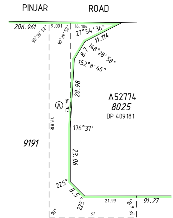
ENLARGEMENT 'E1' Not to Scale
